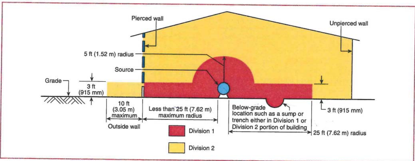
EXHIBIT 500.1 An example of an area classification drawing.
